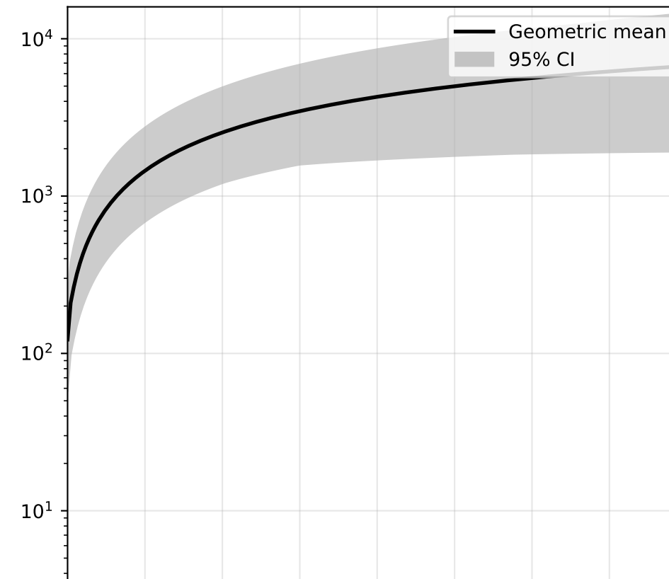
Emission: continental riverwater
