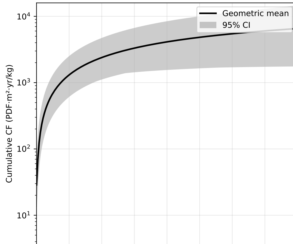
Emission: continental seawater surface
